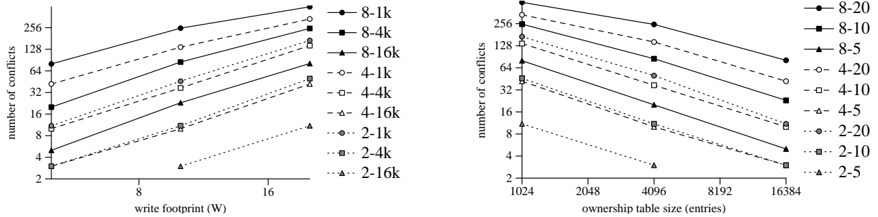
Figure 5: Closed system simulations. Data plotted for <concurrency, table size> and <concurrency, write footprint> pairs, respectively.
