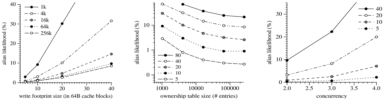
Figure 2: Aliasing likelihood as a function of data footprint (a), ownership table size (b), and concurrency (c). (a,b) data shown for concurrency C = 2 for data footprints [5, 10, 20, 40, 80] and ownership table sizes [1k, 4k, 16k, 64k, 256k] entries. (c) data shown for footprint sizes [5, 10, 20, 40] and an ownership table of size N = 64k .
