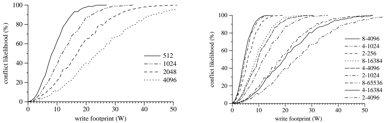
Figure 4: Validation of the model through statistical simulation. (a) conflict likelihood scales quadratically with the transaction footprint (x-axis) and inversely with the ownership table size (512-4096 entries). b) conflict likelihood asymptotically scales quadratically with the concurrency, but at low concurrency the linear term of C(C - 1) is non-negligible; data plotted for <concurrency, ownership table size> pairs.
