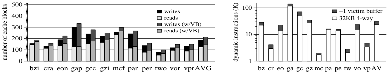
Figure 3: Average maximum footprint size (a) and dynamic instruction count (b) for transactions overflowing a 4-way set associative 32KB cache with 64-byte blocks. a) Typically overflow occurs when 2/5ths of the cache’s 512 blocks have been touched. A single entry victim buffer results in a 16% increase in hardware supported transaction footprint size. b) Size (in thousands of dynamic instructions) of transactions at the time of overflow.
