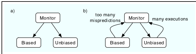
Figure 4. A finite-state machine model for branch behavior characterization.
