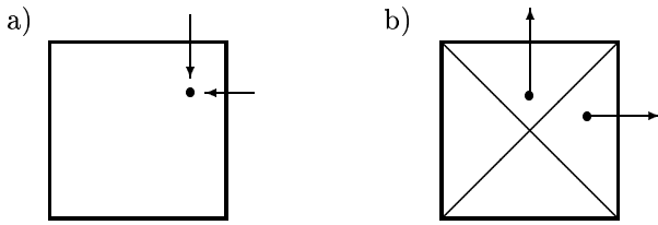
Figure 2: Generation of contact forces using volumes (the small dot represents the haptic interface point). a) Two possible paths to reach the same location in a square are shown; without a history we do not know which path was taken. b) Vector field method (in 2 dimensions): subdivide the square’s area and assume that the user entered from the closest edge. The force vectors are normal to the edge and proportional to distance penetrated. This method is easily expanded to 3 dimensions.
